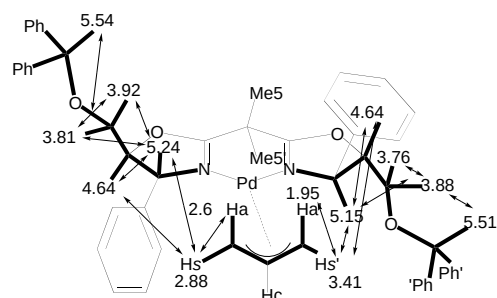
Figure 3. Relevant NOE contacts from NOESY experiment of 8c (proton chemical shifts in ppm).
