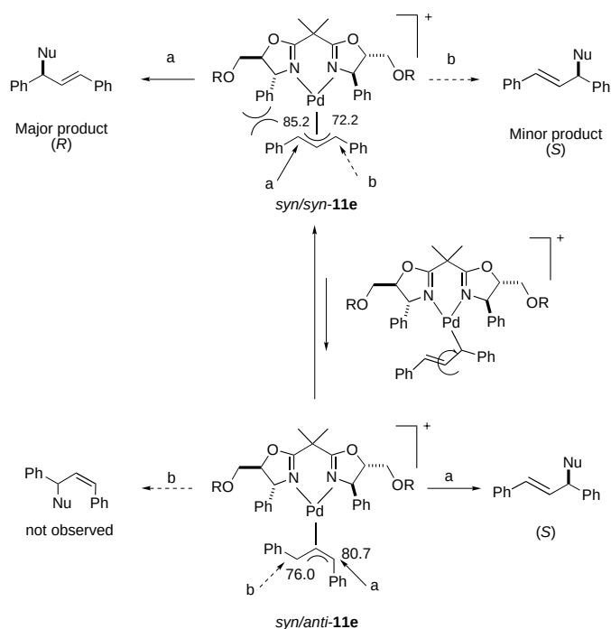
Scheme 7. Selectivity of the dimethyl malonate attack on the terminal allylic carbon atoms of type- 11 species.
