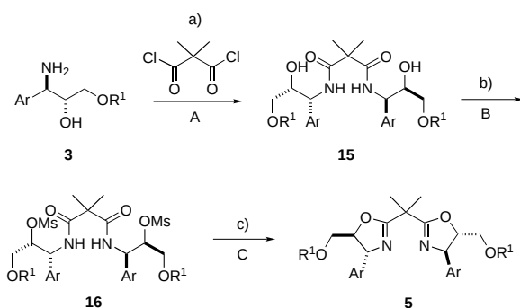
Scheme 3. Three-step synthesis of bis(oxazolines) 5 from amino alcohols 3 . a) Et 3 N, CH 2 Cl 2 ; RT, 20 h; b) 2.2 equiv MsCl, 4.4 equiv Et 3 N, CH 2 Cl 2 , 0 °C → RT, 2 h; c) 5% KOH/MeOH, RT, 15 h.
