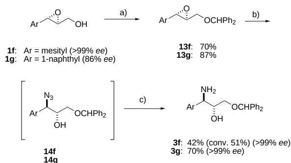
Scheme 2. Synthesis of chiral amino alcohols 3 from epoxyalcohols 1 . a) NaH, DMF, BrCHPh 2 , 0 °C, 17 h; b) NaN 3 , LiClO 4 , CH 3 CN, 55 °C, 24 h; c) NaBH 4 , THF/MeOH, 55–60 °C, 22 h.
