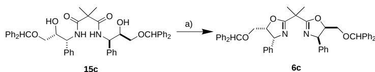
Scheme 4. Synthesis of bis(oxazoline) 6c from bis(hydroxyamide) 15c . a) \text{Bu}_2\text{SnCl}_2 , xylene, reflux, 48 h.
