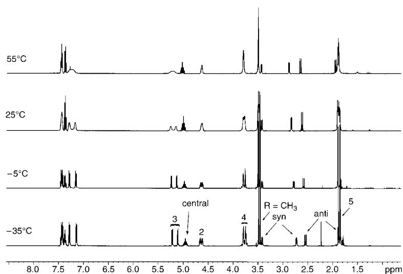
Figure 2. Variable temperature ^1\text{H} NMR spectra of 8a .
