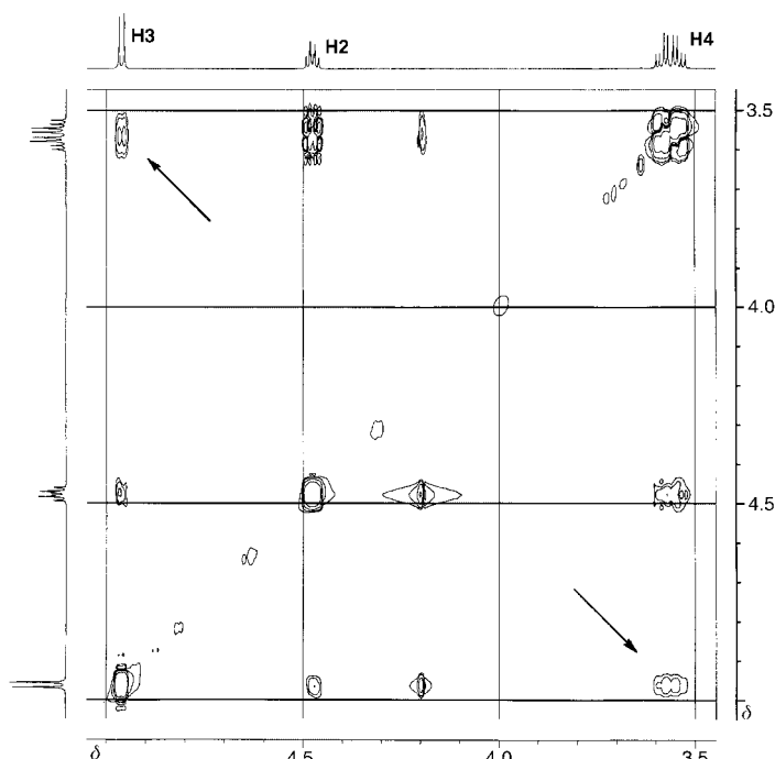
Figure 1. Part of the NOESY spectrum (3.5–5 ppm) of 5c (arrows indicate NOE contacts between H3 and H4 protons).
